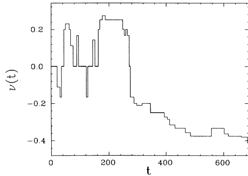
FIG. 1. Type of a chaotic orbit for the standard map at K=1.2 , with initial condition (x_0, p_0) = (0.5001, 0.0) . The type is represented here by the winding number \nu = m/n of the resonance visited as a function of time t . This is a steplike function, assuming a constant value m_r/n_r in a time interval of length q_r n_r [ q_r rotations in resonance (m_r, n_r) ]. This function is plotted up to the first crossing time of a golden-mean cantorus with \nu = (\sqrt{5} - 3)/2 .
